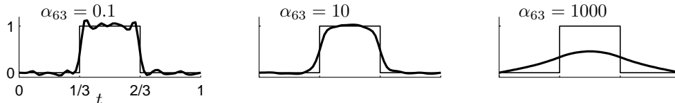
Figure 3. Gaussian MAP estimates with three different choices of \alpha_{63} . The function u(t) is plotted with a thin line. Left: too small \alpha_{63} . Middle: satisfactory solution. Right: too large \alpha_{63} .
