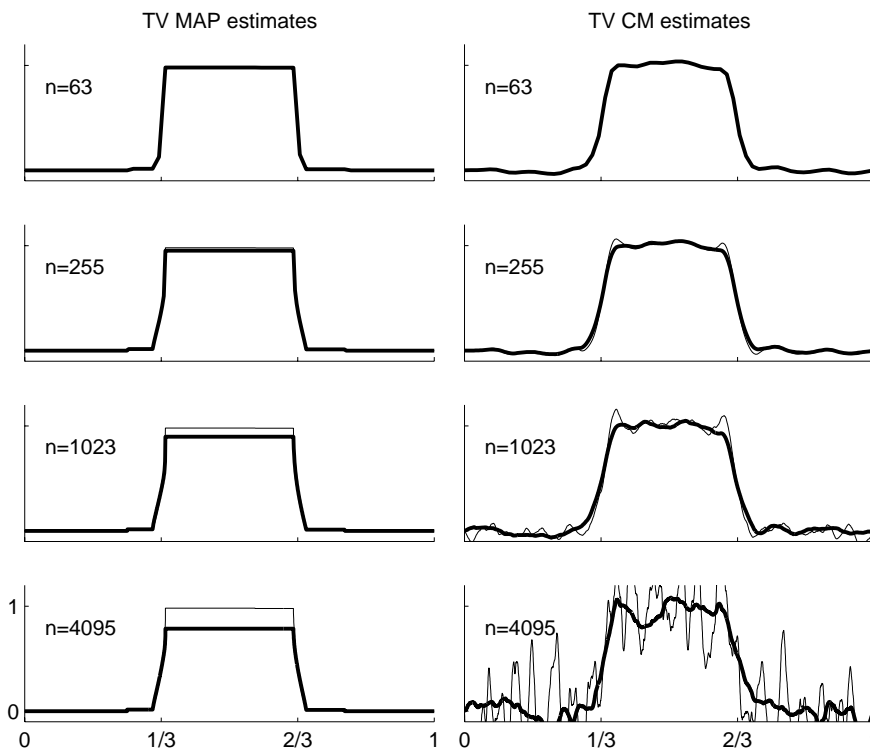
Figure 4. In all the plots in this figure, the coordinate axes limits are the same to allow easy comparison. Left column: MAP estimates for the TV prior with parameter \alpha_n = 135 (thin line) and \alpha_n = 16.875\sqrt{n+1} (thick line). Right column: CM estimates for the TV prior with parameter \alpha_n = 135 (thin line) and \alpha_n = 16.875\sqrt{n+1} (thick line).
