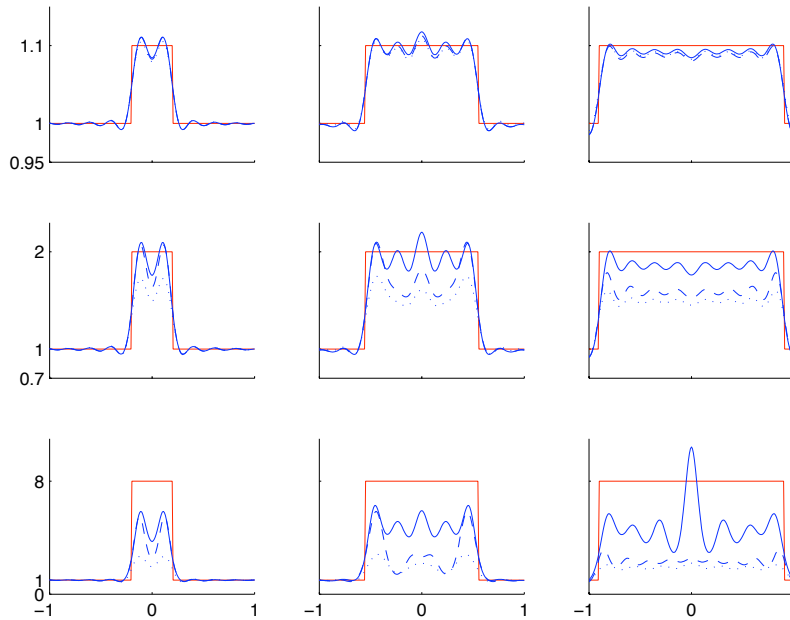
Figure 1. Actual (red) and reconstructed conductivity profiles from Calderón's method (dotted), \mathbf{t}_R^{\text{exp}} (dashed) and \mathbf{t}_R^B (solid) with R = 15 for the conductive discontinuous examples. The last two reconstructions in the third row were computed with R = 12 .
