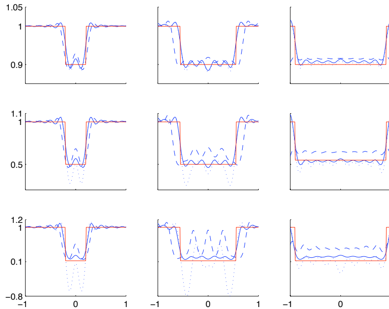
Figure 2. Actual (red) and reconstructed conductivity profiles from Calderón's method (dotted), \mathbf{t}_R^{\text{exp}} (dashed) and \mathbf{t}_R^{\text{B}} (solid) with R = 15 for the resistive discontinuous examples. The last reconstruction in the third row was computed with R = 12 . Note that the last row of examples has the highest contrast; the scale of the plots were chosen to accommodate the Calderón reconstructions.
